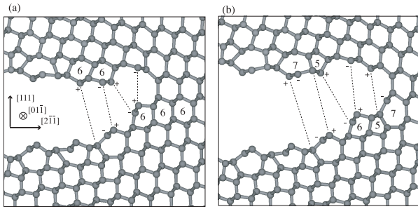
FIG. 5: Step formation process on (111) cleavage plane. The step is classified into the '[211]-' or 'via-(111)-plane'-type step (See Fig. 2(f)). Two snapshots with a time interval of approximately 0.6 ps are shown. The dashed lines indicate the initial (crystalline) bonds. The '+' and '-' symbols on atoms indicate excess and deficit electron populations, respectively.
