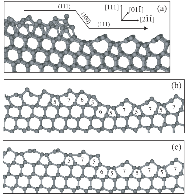
FIG. 6: (a) (111) cleaved surface with '[211]-' or 'via-(100)-plane'-type step. The arrow indicates the cleavage propagation direction. (b)(c): Two 'slices' of (a) (See text for details).
