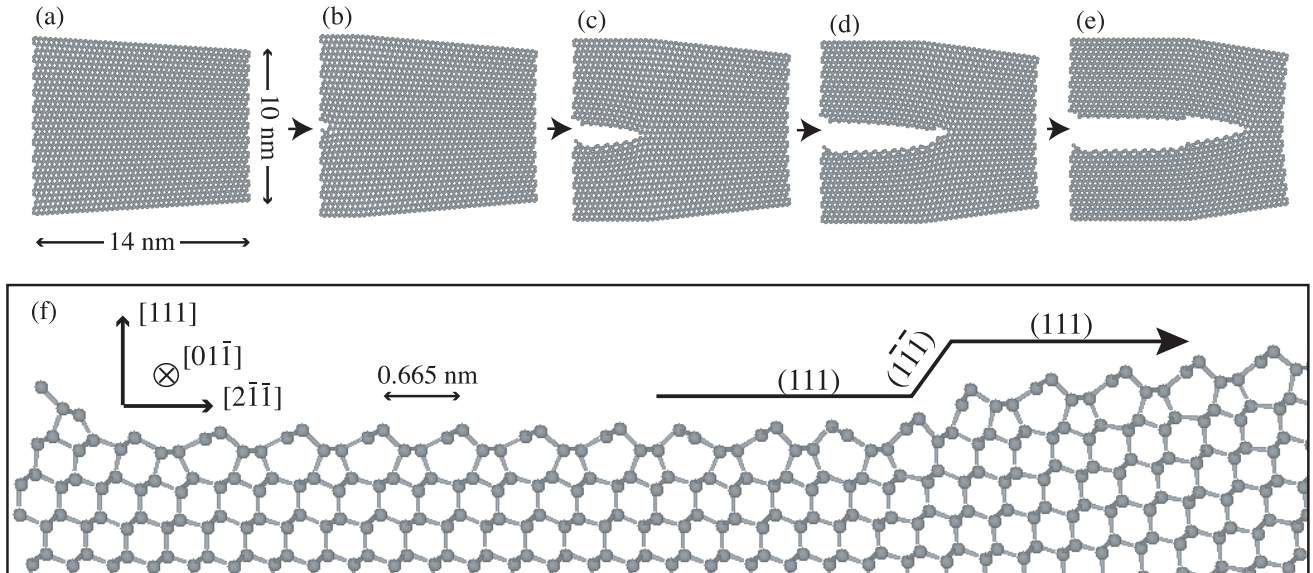
FIG. 2: Cleavage process of silicon with (111) - (2 \times 1) cleaved surface. (a)-(e): Successive snapshots with a time interval of approximately 2 ps. (f): A part of the lower cleavage surface shown in the snapshot (e). A step is found and is classified into the ‘ [\bar{2}11] -type’ or ‘via- (1\bar{1}\bar{1}) -plane type’ that can be decomposed into the successive bending of cleavage planes as (111) \rightarrow (1\bar{1}\bar{1}) \rightarrow (111) .
